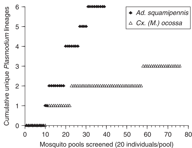
Fig. 2 The cumulative numbers of unique Plasmodium cytochrome b lineages sequenced from pools of individual mosquitoes of two mosquito species, Aedeomyia squamipennis and Culex (Melanoconion) ocossa .
